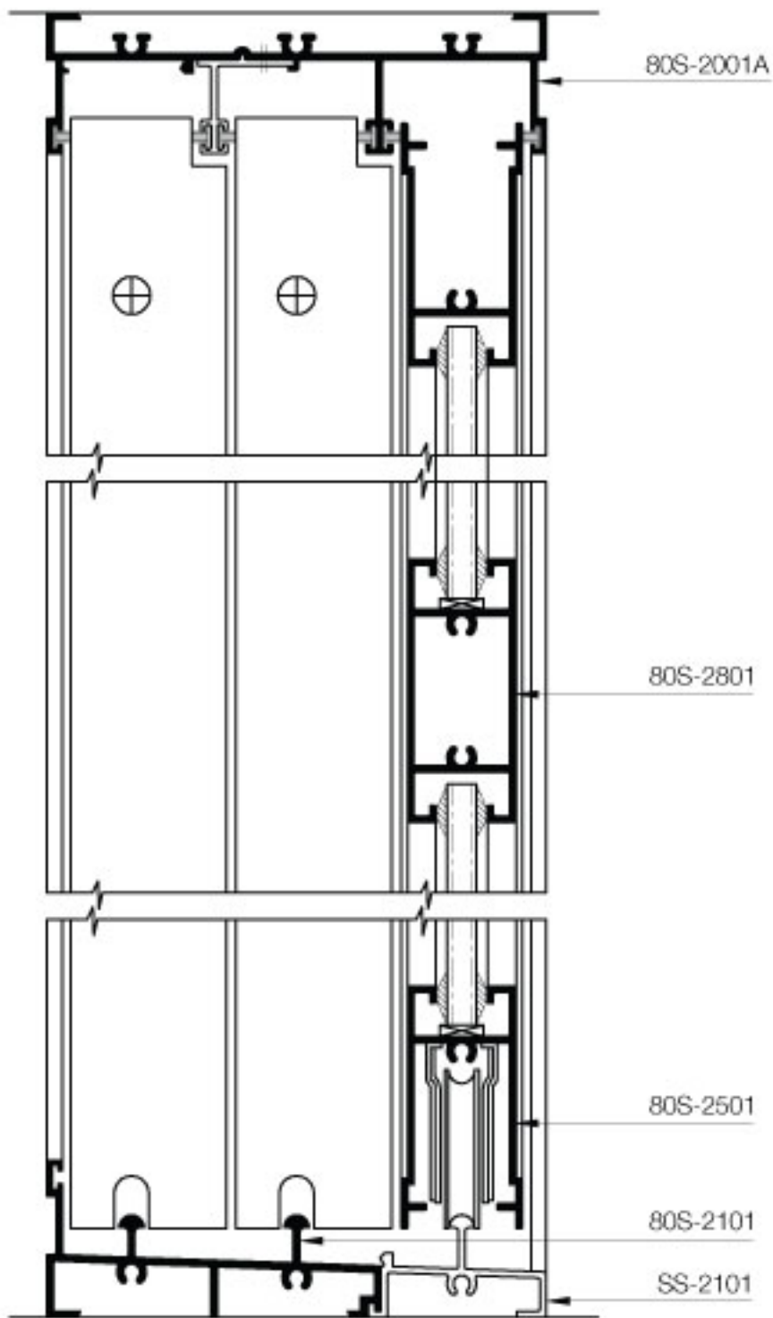
SECTION: A-A
