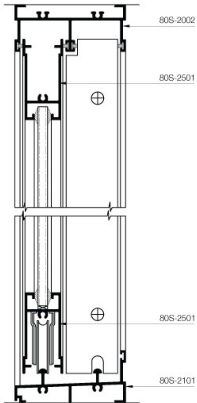
SECTION: A-A
