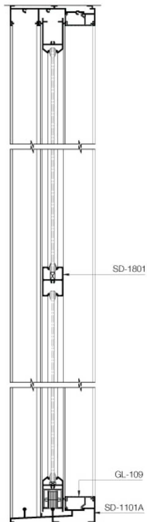
SECTION: B-B
