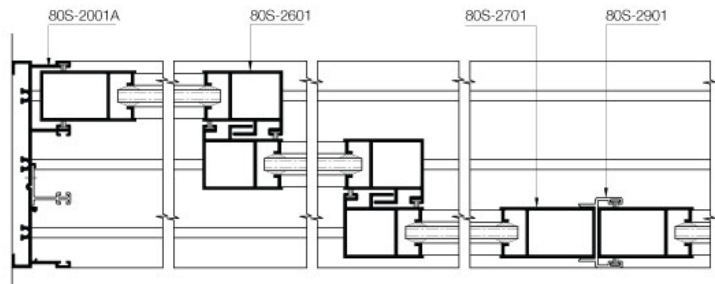
SECTION: B-B
