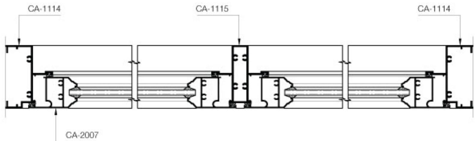
SECTION: B-B
