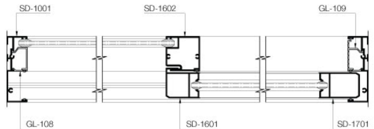
SECTION: C-C
