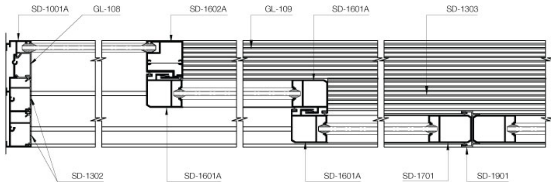
SECTION: D-D
