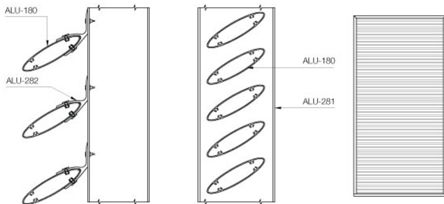
Sun Louvre using Bird Mouth Bracket
