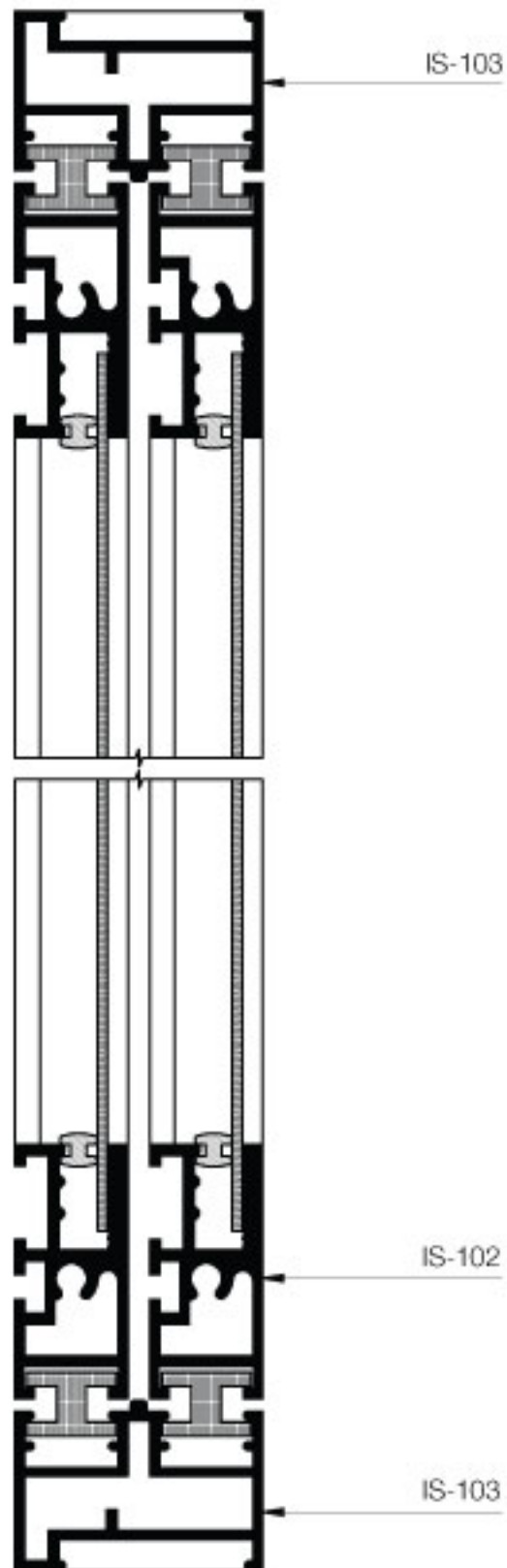
SECTION: A-A
