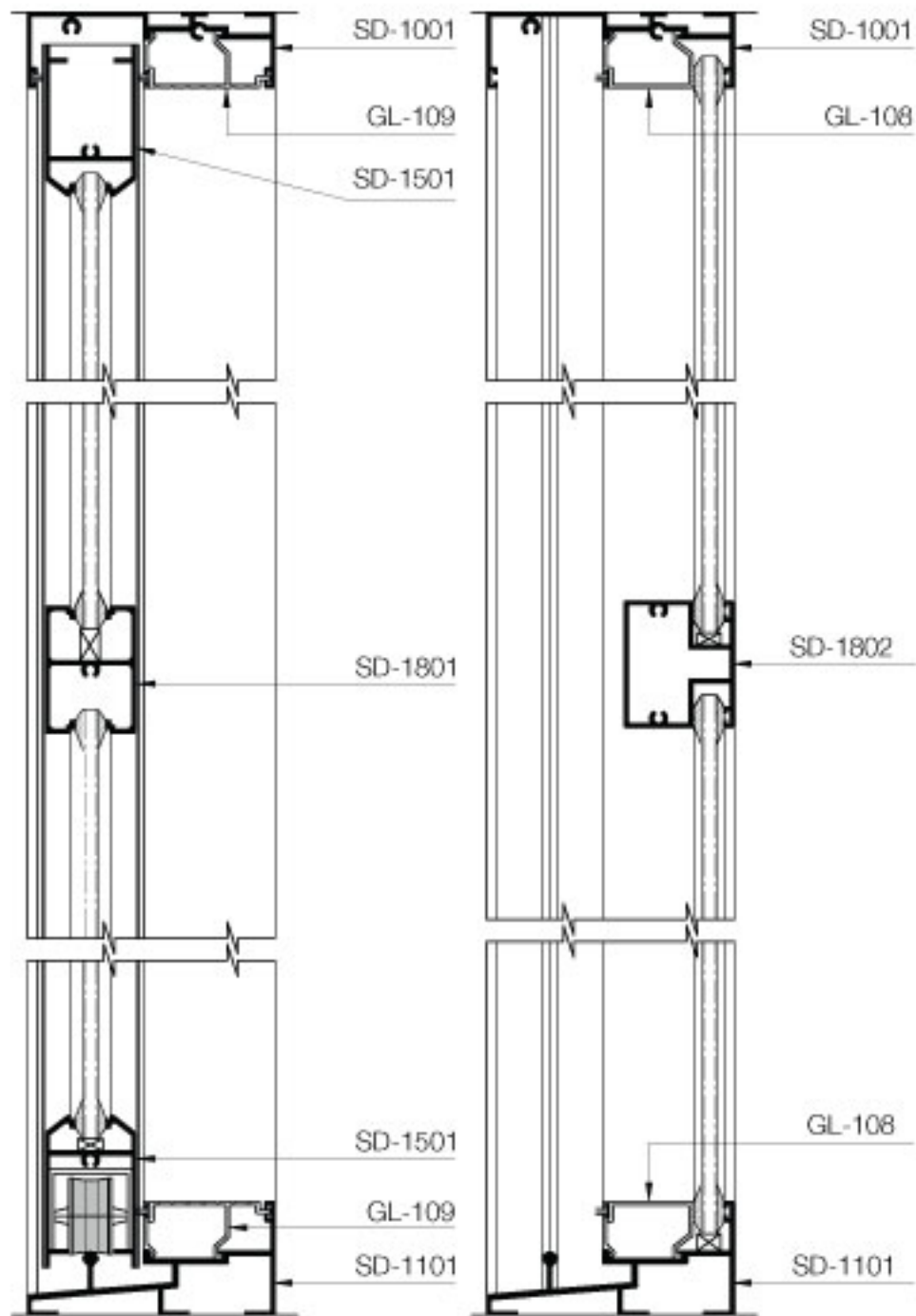
SECTION: A-A
