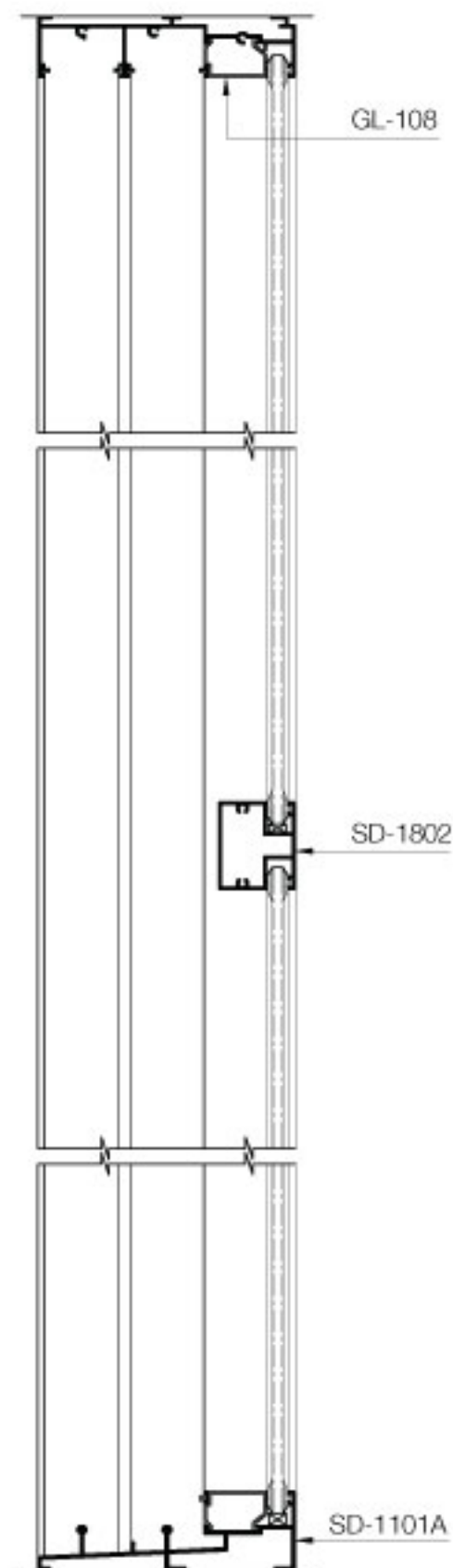
SECTION: C-C
